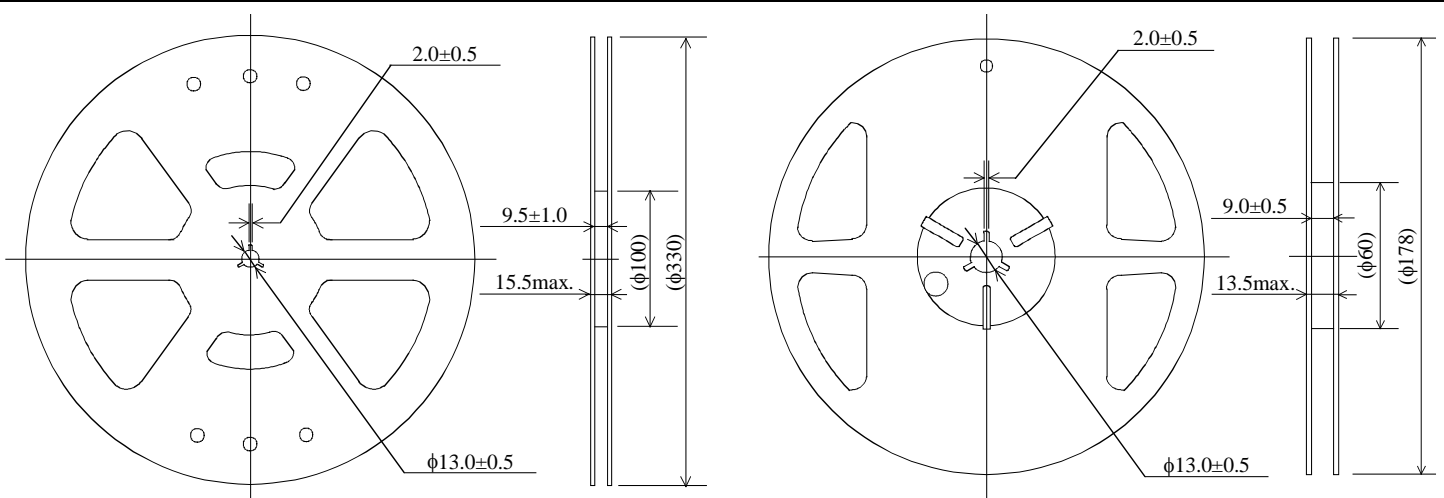
SAWEN881MCM2F00R00 ... 10000pcs/reel
