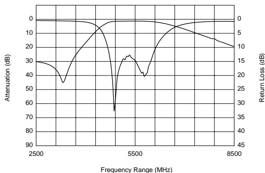
Frequency Characteristics
