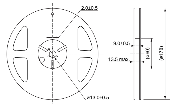
\phi 178 Reel Dimension
