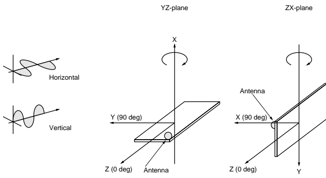
Antenna gain (3D measurement)
