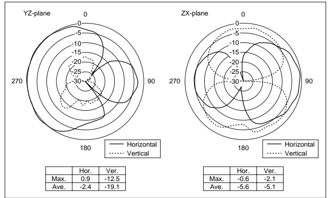
Radiation Pattern
