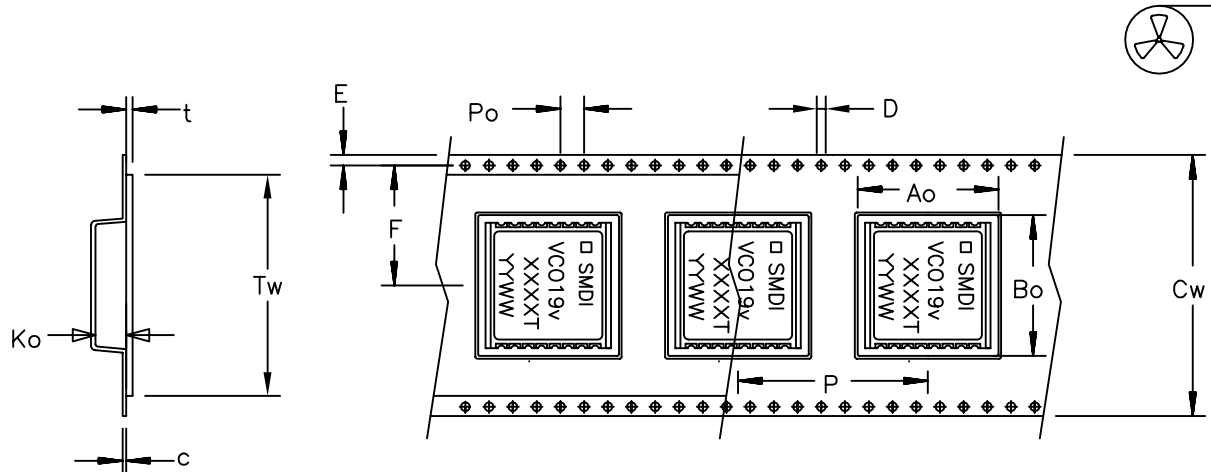
T-PACKAGE TAPE DIMENSIONS (ALL DIMENSIONS IN MM)
