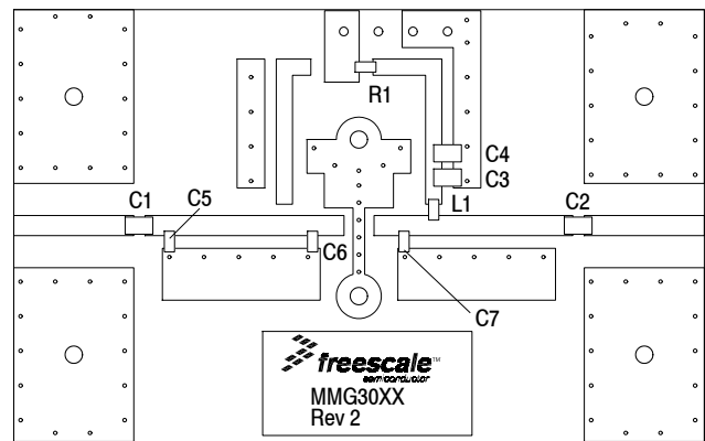
Figure 25. 50 Ohm Test Circuit Component Layout
