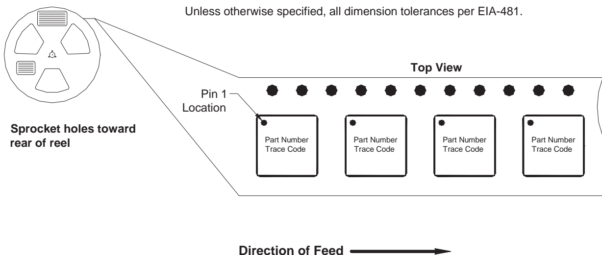
Figure 1. 2mm x 2mm (Carrier Tape Drawing with Part Orientation)
