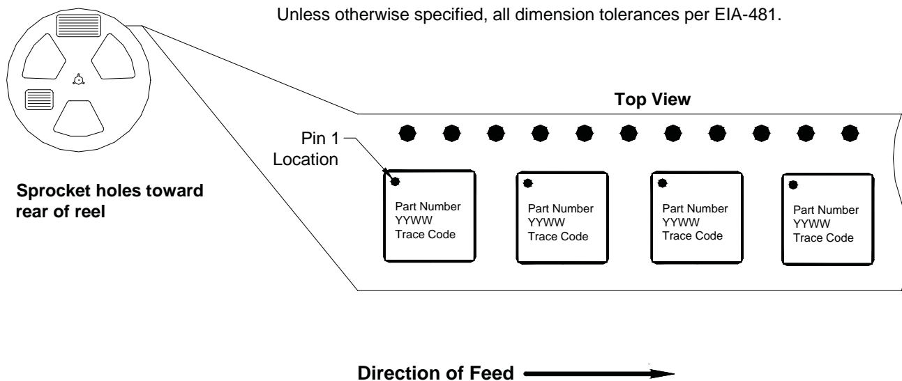
Figure 1. 6.000mm x 6.000mm (Carrier Tape Drawing with Part Orientation)
