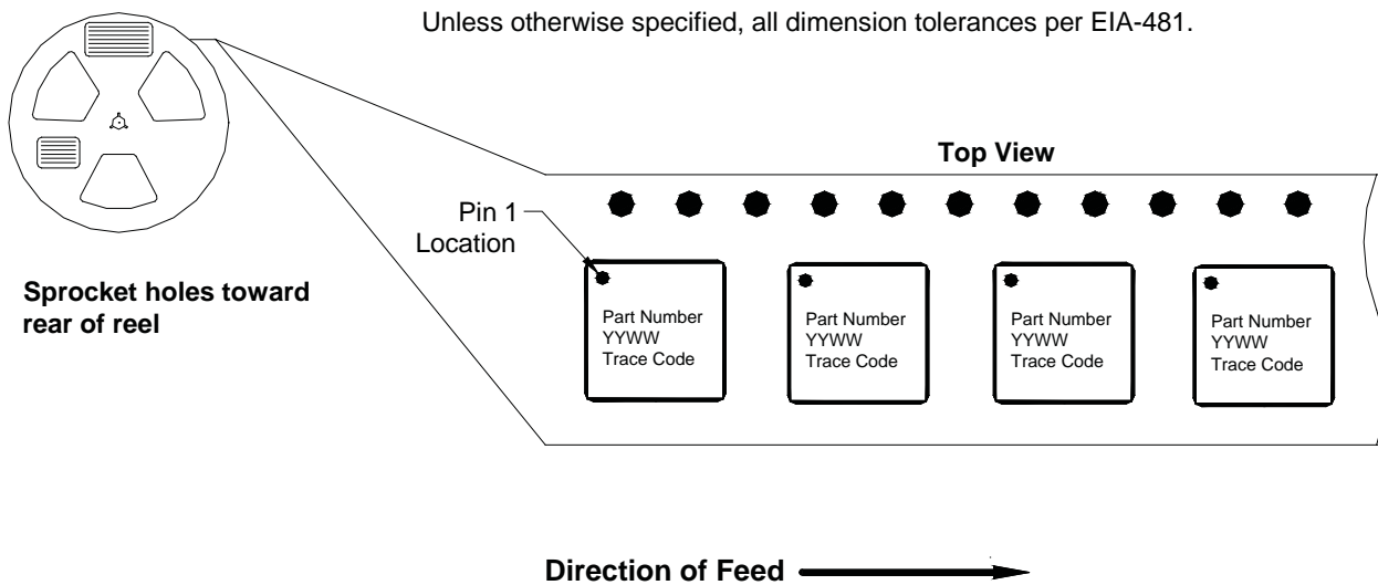
Figure 1. 7.000mm x 7.000mm (Carrier Tape Drawing with Part Orientation)
