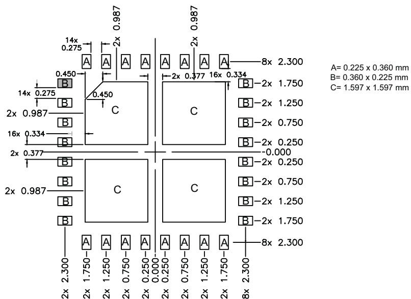
Figure 2. Stencil Recommendation
