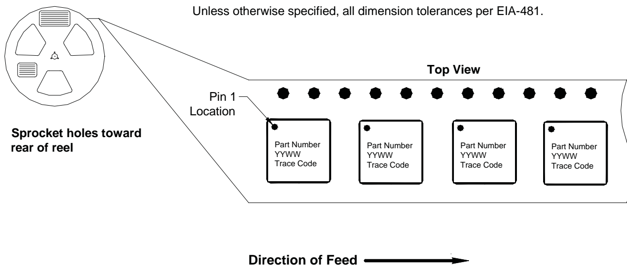
Figure 1. N6.000mm x 6.000mm (Carrier Tape Drawing with Part Orientation)
