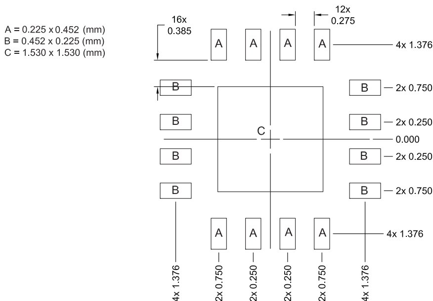
Figure 2. Stencil Recommendation
