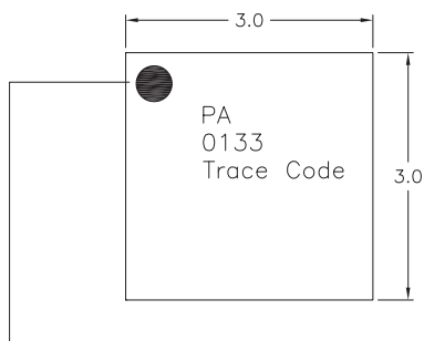
Pin 1 Indicator
