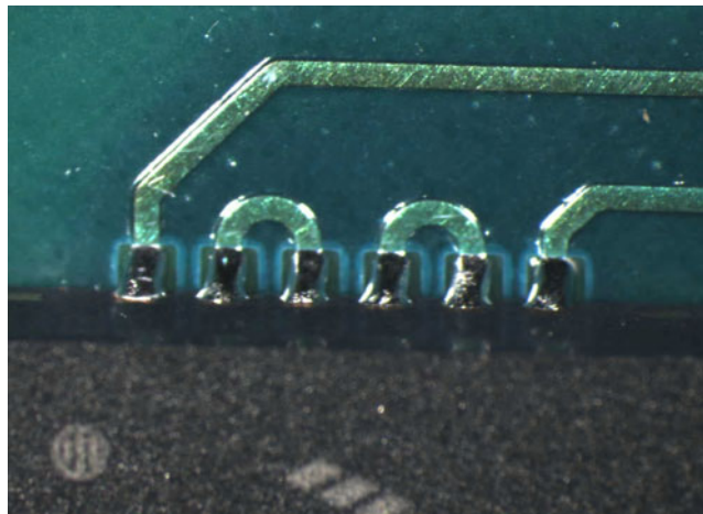
Figure 11. No Solder Balling was Observed for Case 6L-C, d = 0.40 mm, Sn62 Solder (Good Fillets Formed Above the Extended Part of PCB Pads)
