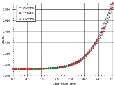
Icc(A) vs. Pout(dBm) -40° C Vcc=5Vdc Vreg=2.85Vdc
