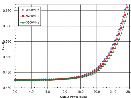
Icc(A) vs. Pout(dBm) 85° C Vcc=5Vdc Vreg=2.85Vdc
