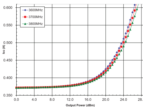
Icc(A) vs. Pout(dBm) 25° C Vcc=5Vdc Vreg=2.85Vdc
