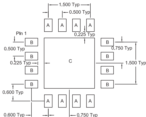
PCB METAL LAND PATTERN
