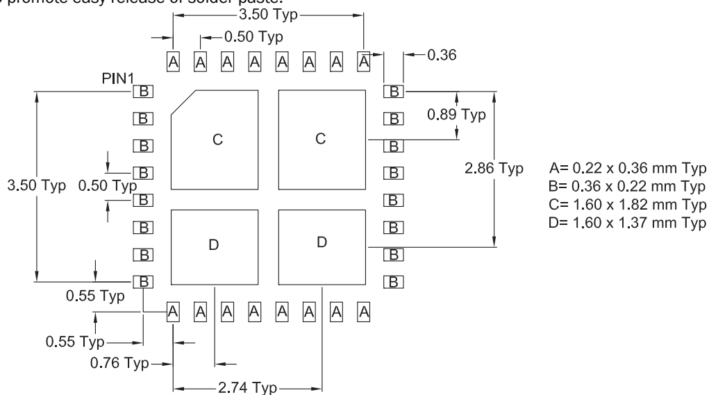
Figure 2. Stencil Recommendation
