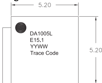
Pin 1 Indicator
