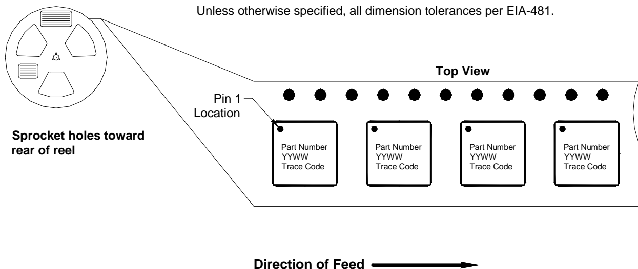
Figure 1. 5.2mm x 5.2mm (Carrier Tape Drawing with Part Orientation)
