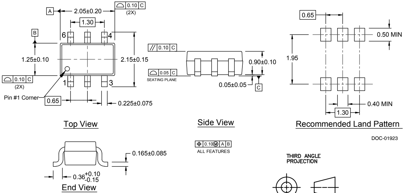
Figure 15. Package Drawing 6-lead SC-70
