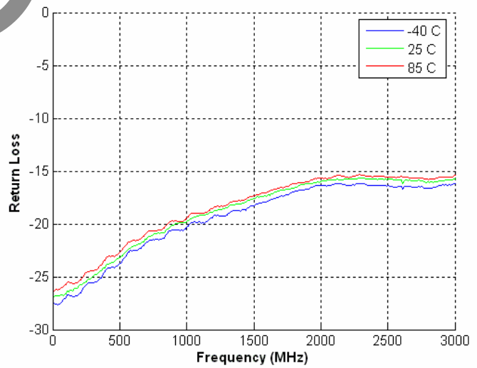
Figure 17. Return Loss: RFC-RF1 @ 3 V
