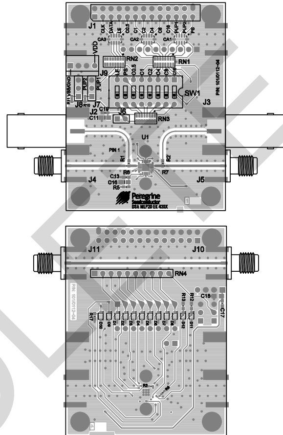
Figure 15. Evaluation Board Layout
