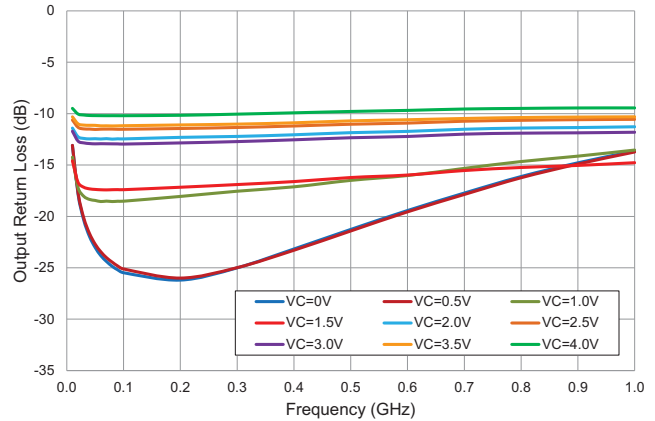
Output Return Loss versus Voltage Control RFSA3013, RF 1GHz, V_{DD}=5V
