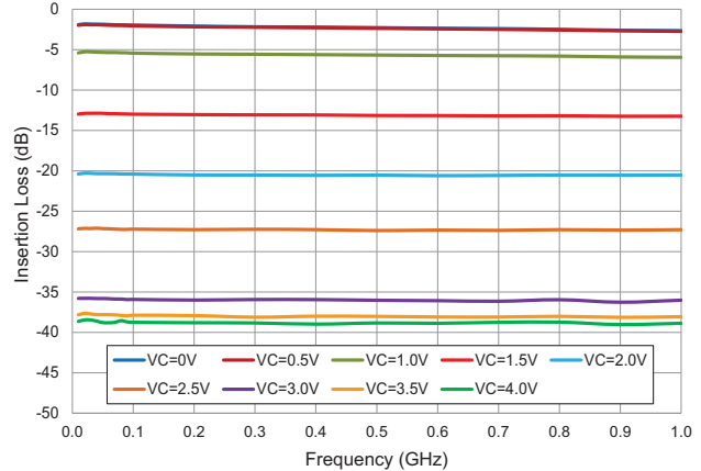
Insertion Loss versus Frequency RFSA3013, V_{DD}=5V , Temp=+25°C
