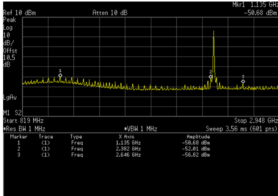
Figure 11. Power Setting 0x0C Radiated Broadband Spectrum.
