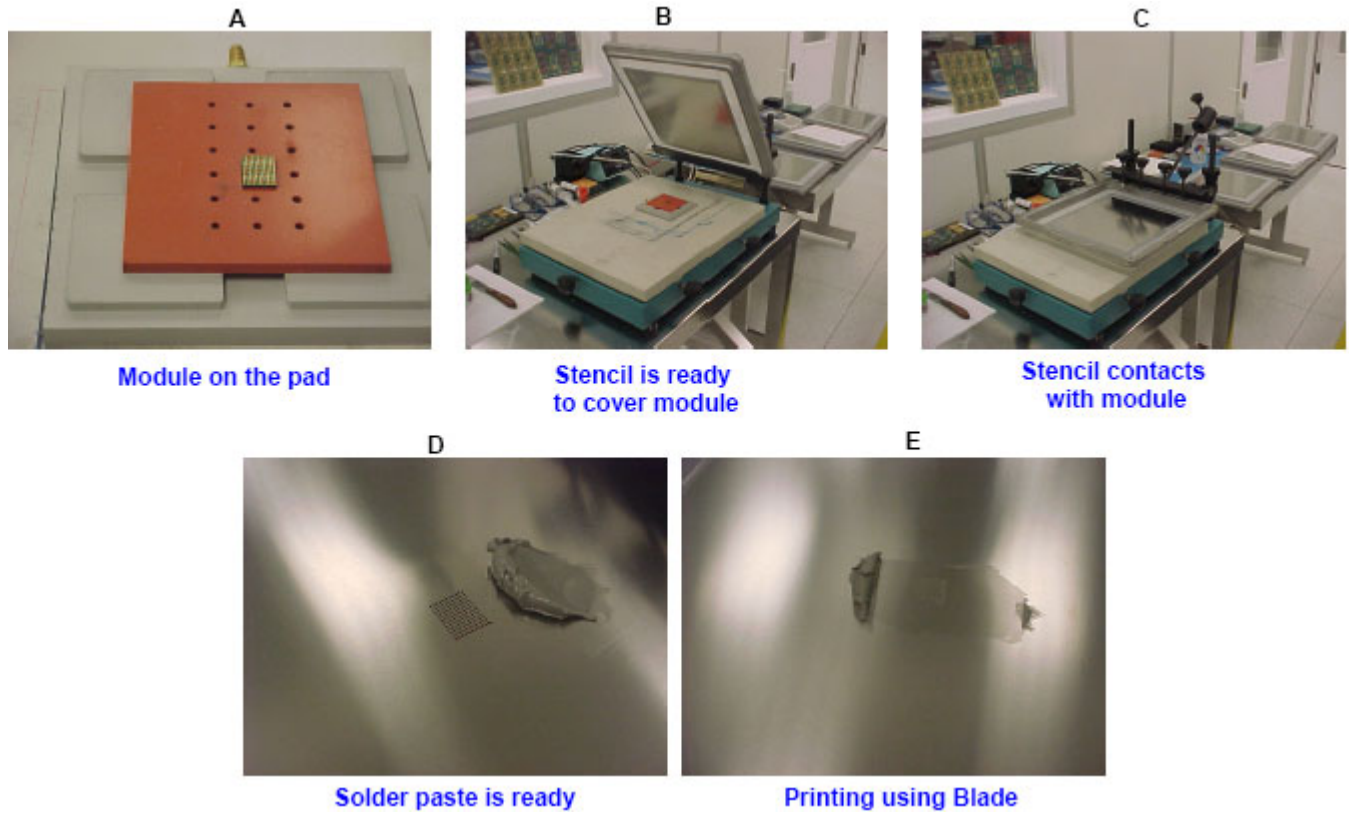
Figure 8. Pre-tinning an LGA
