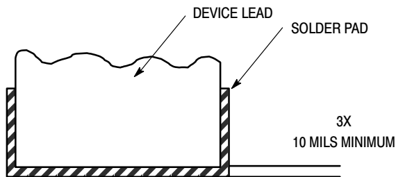
Figure 9. Pad Size for Gate and Drain Side Leads
