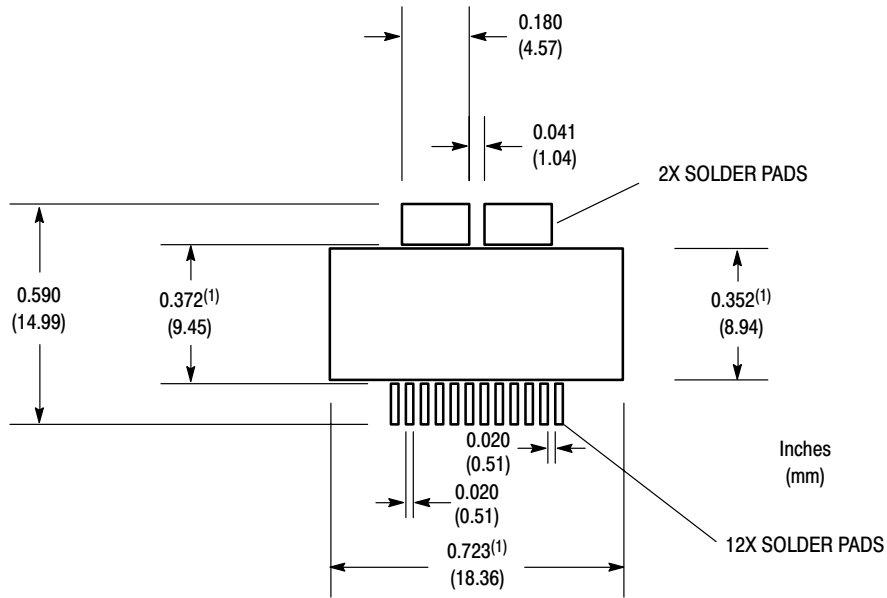
Figure A-9. Case 1618 (TO-270 WB-14)
