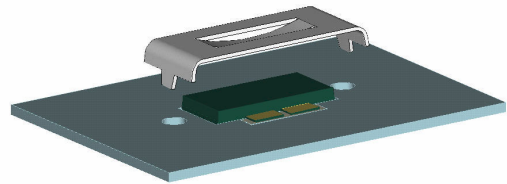
Figure 14. Typical Fixture or Clips for use During Solder Reflow
