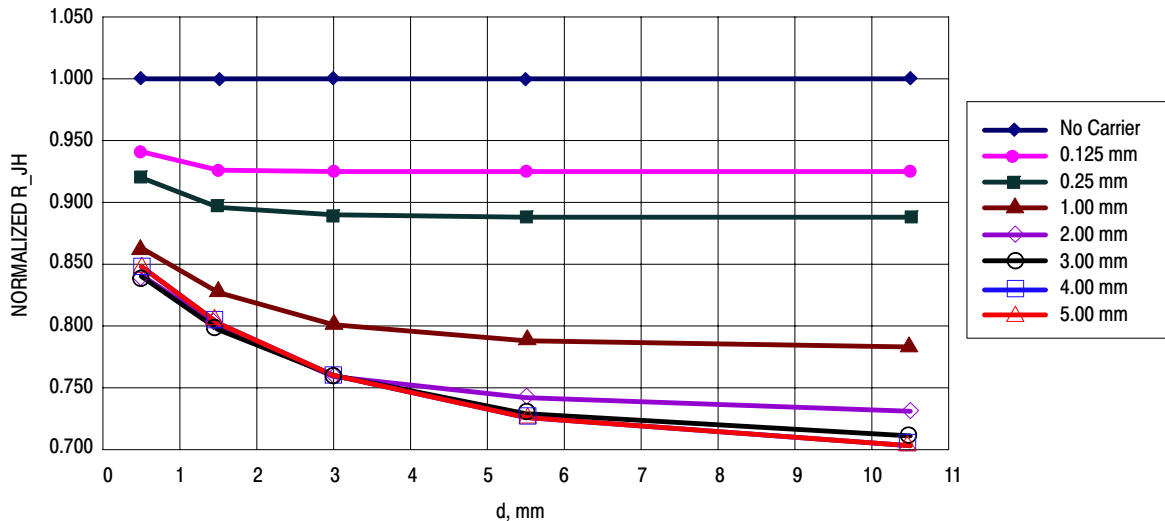
Figure 7. Parametric Study Results for Aluminum Carrier
