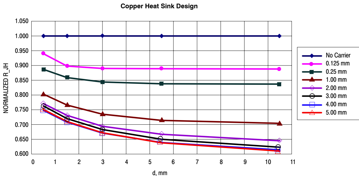
Figure 6. Parametric Study Results for Copper Carrier
