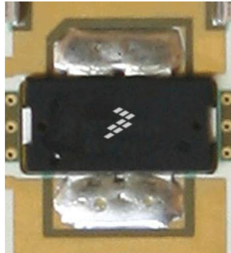
Figure 1. Typical Application of Freescale RF Power Device in Over-Molded Plastic Packages Soldered to a PCB as Well as to Carrier
