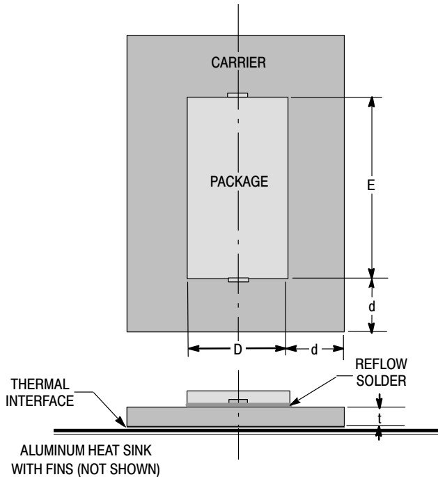
Figure 5. Typical Carrier Inserted Between Device and Aluminum Heat Sink
