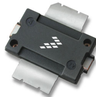
Figure 2. Typical RF Power Plastic Device Compatible for Solder Reflow Process (Case 1265, TO-270-2)
