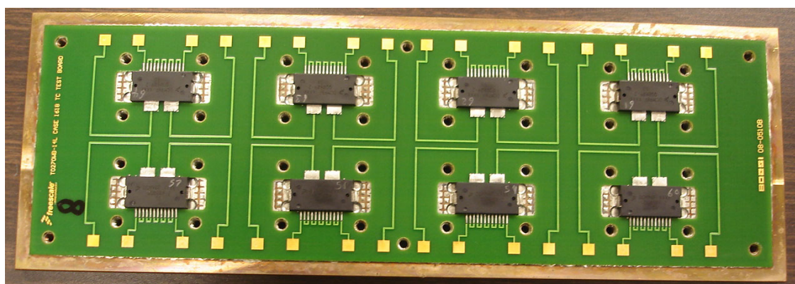
Figure 10. Example of One-Pass Soldering of PCB Device and Carrier
