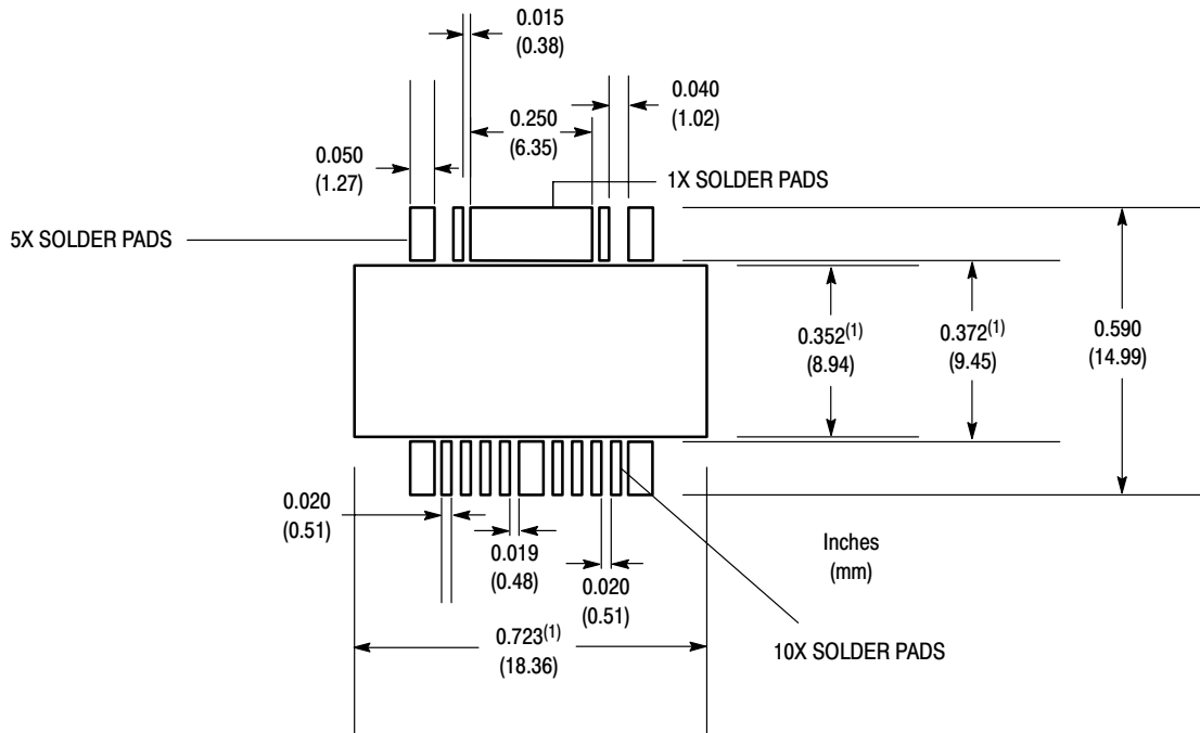
Figure A-11. Case 1886 (TO-270 WB-16)
