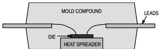
Figure 3. Over-Molded Plastic Package Construction for Power Devices
