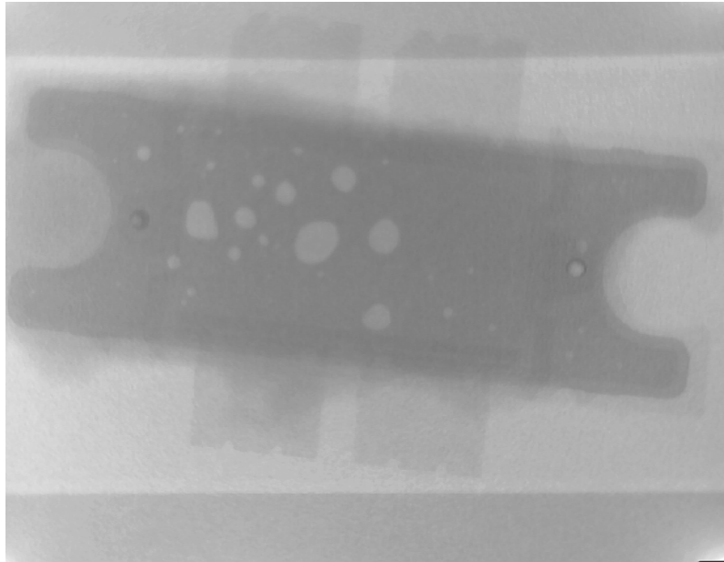
Figure 15. X-Ray Image Showing Voids in Solder Attach for TO-272WB-4 Mounted on 0.210" (5.33 mm) Thick Copper Plate. (The image was taken on a FocalSpot, Inc. system. Used with permission.)
