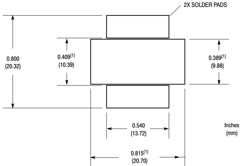
Figure A-12. Case 2021 (OM-780-2)
