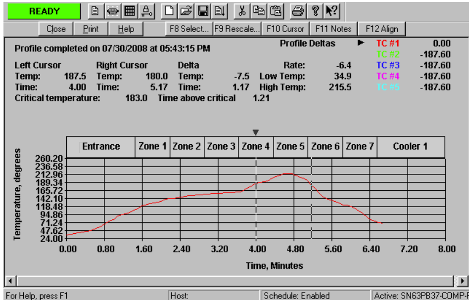
Figure 13. Typical Solder Reflow Profile for Eutectic SnPb Solder
