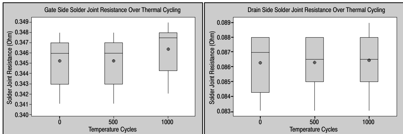
Figure 17. Box-and-Whisker Plot of Electrical Resistance of Gate Side and Drain Side Daisy Chain Circuit Indicating no Shift in Resistance or Solder Joint Cracking
