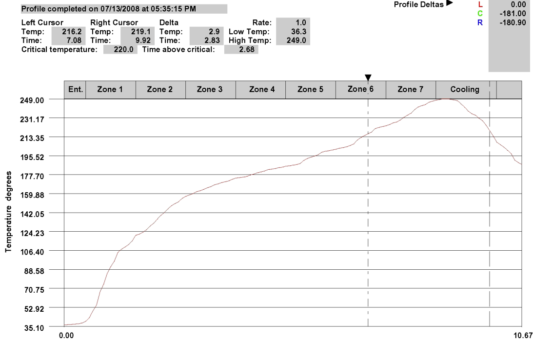
Figure 11. Solder Reflow Profile for One-Pass Pb-Free (SnAgCu) Soldering of OMP Devices with PCB and Carrier Shown in Figure 10
