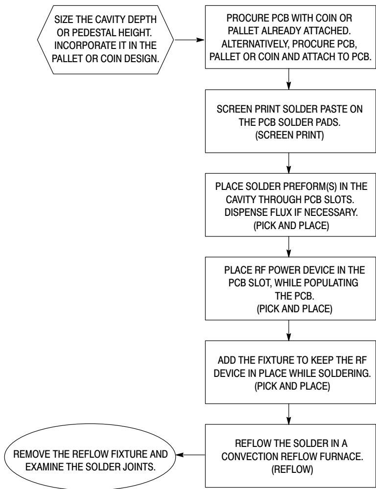
Figure 12. Typical Process Flow for Assembly of PCB using Solder Reflow Method
