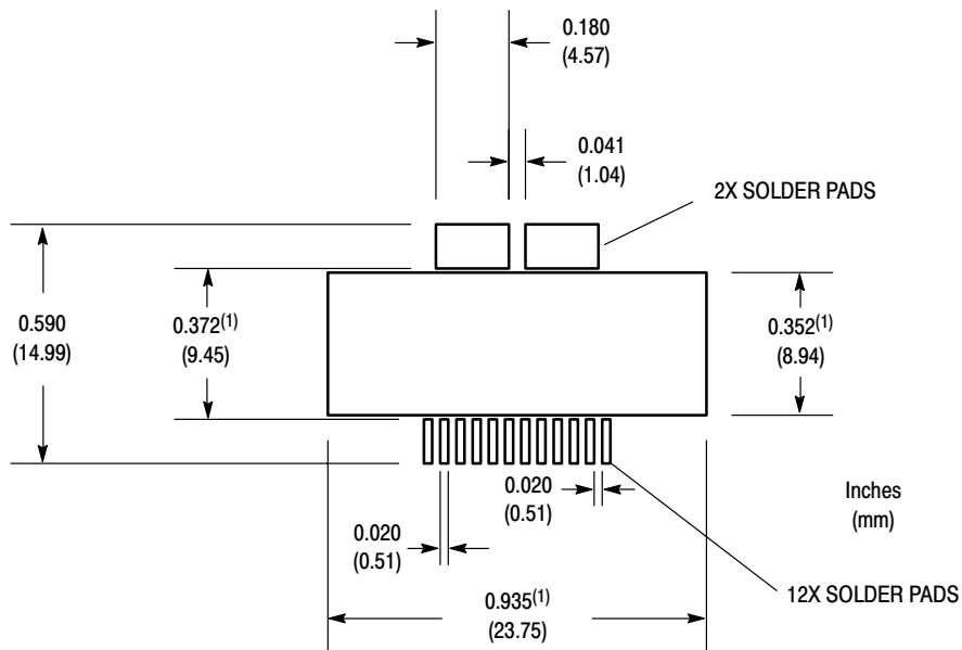
Figure A-8. Case 1617 (TO-272 WB-14)
