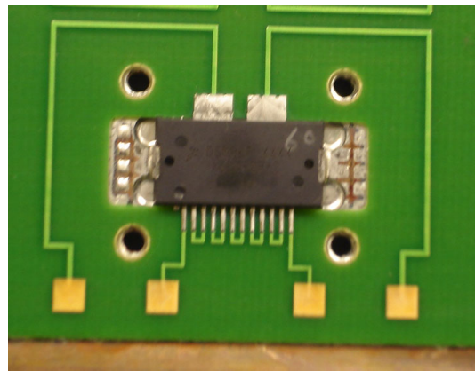
Figure 16. Close-Up View of one of the Daisy-Chained Devices Soldered to a Copper Carrier and the PCB
