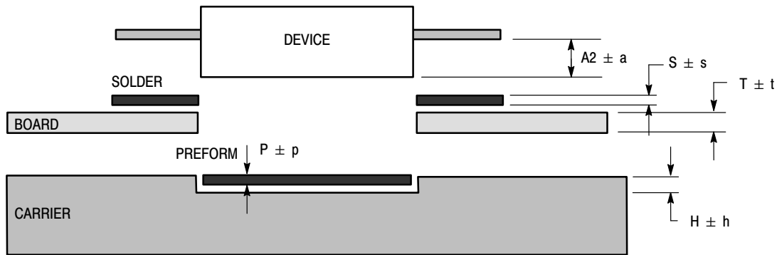
Figure 8. Exploded View Showing Criteria and Tolerances for Calculating Cavity Dimensions
