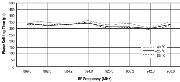
Figure 14. Phase Settling Time vs Frequency and Temperature
