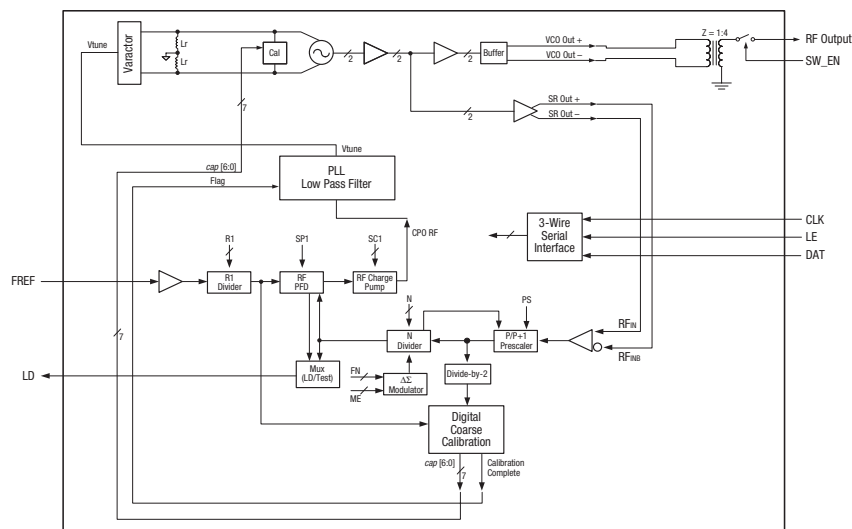
Figure 1. SKY73112-11 Functional Block Diagram
