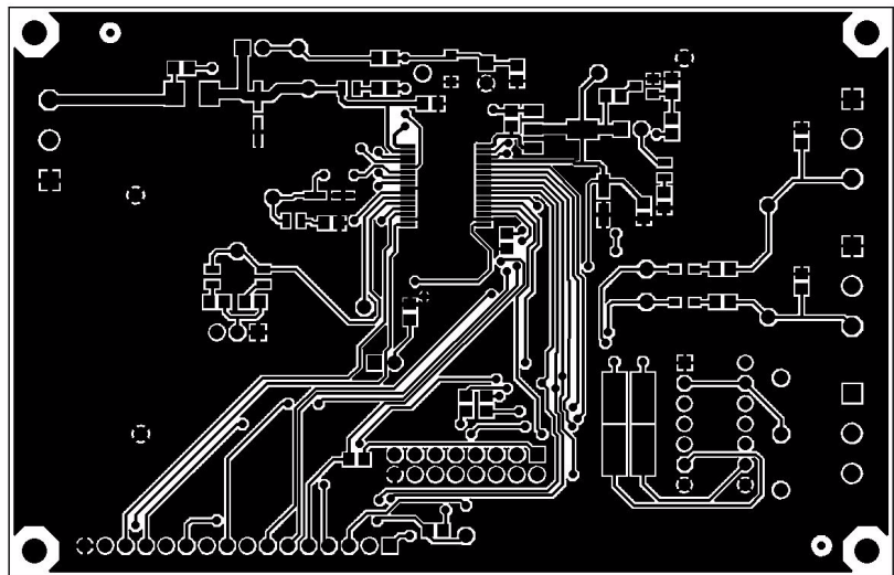
Figure 12. Top Side Layer
