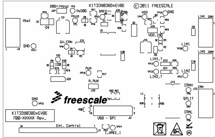
Figure 11. Assembly Drawing
