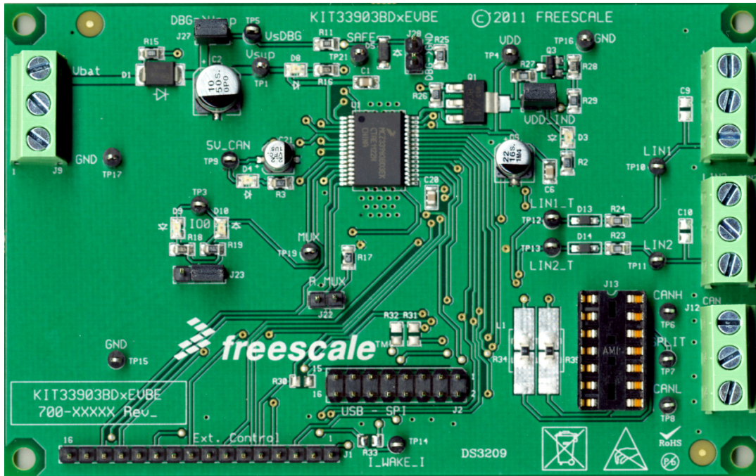
Figure 1. KIT33903BD5EVBE/KIT33903BD3EVBE Evaluation Boards
