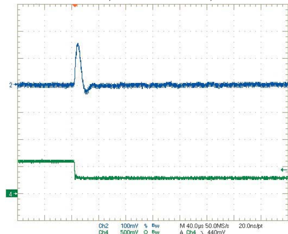
Step Load Transient Response (Vin=12V, Vout=0.591V, Load=0, Iout=3A to 1.5A) Trace 2=Vout, 100 mV/div. Trace 4=Iout, 2.5A/div.
