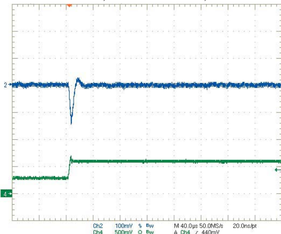
Step Load Transient Response (Vin=12V, Vout=0.591V, Load=0, Iout=1.5A to 3A) Trace 2=Vout, 100 mV/div. Trace 4=Iout, 2.5A/div.
