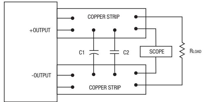
C1 = 1\mu\text{F} CERAMIC C2 = 10\mu\text{F} CERAMIC LOAD 2-3 INCHES (51-76mm) FROM MODULE
