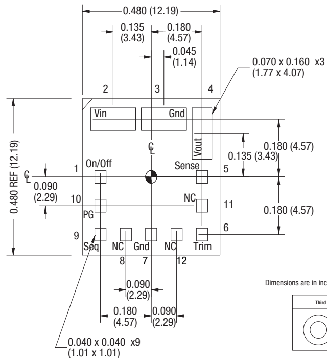
Figure 3. OKL-T/6-W12 Mechanical Outline
