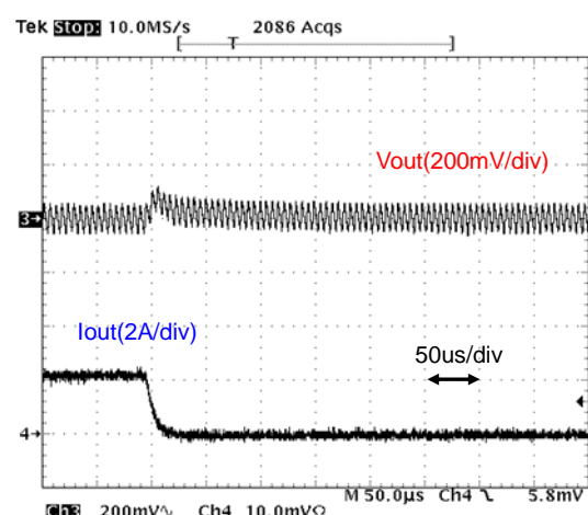
Fig.12-2-36. Load Transient Response (Io= 2A → 0)
