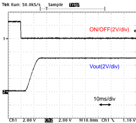
Fig.12-2-15. Start-up Waveform (Io=0A)
