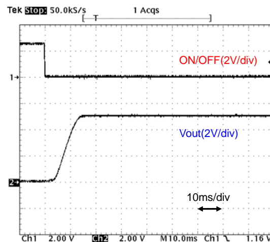
Fig.12-2-4. Start-up Waveform (Io=2A)
