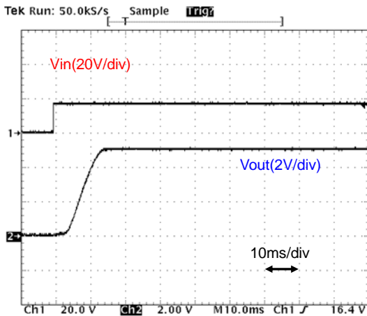
Fig.12-2-1. Start-up Waveform (Io=0A)
