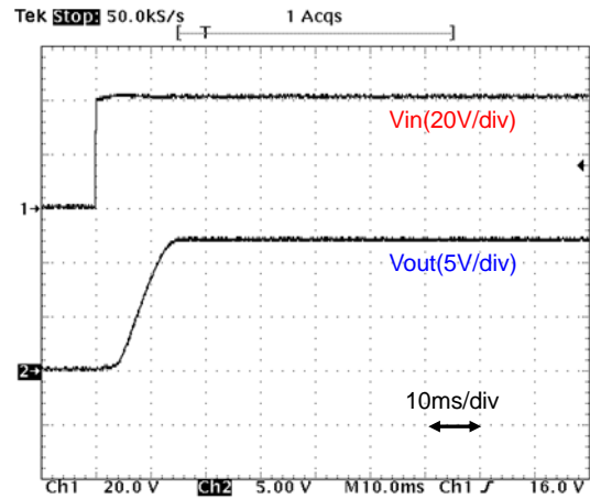
Fig.12-2-32. Start-up Waveform (Io=2A)
