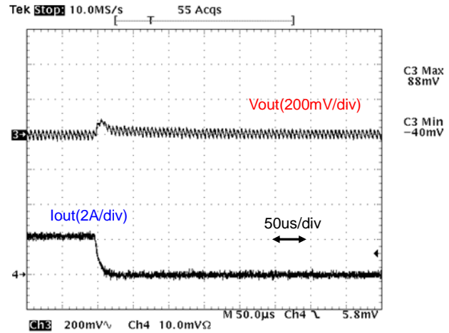
Fig.12-2-18. Load Transient Response (Io= 2A → 0)
