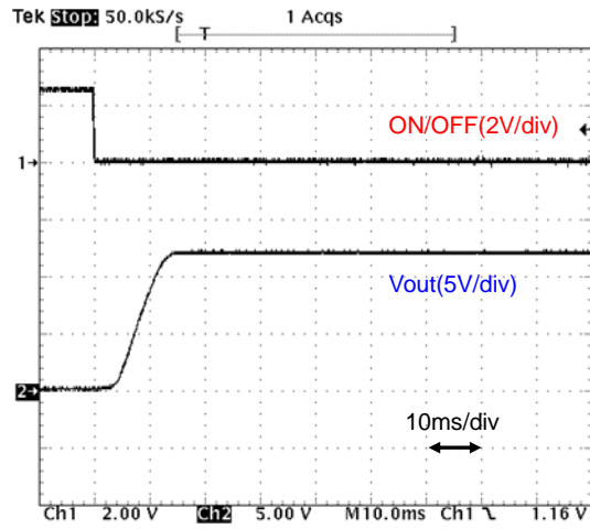
Fig.12-2-22. Start-up Waveform (Io=2A)
