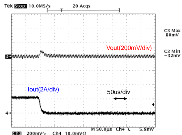
Fig.12-2-6. Load Transient Response (Io= 2A → 0)
