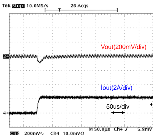
Fig.12-2-23. Load Transient Response (Io= 0 → 2A)
