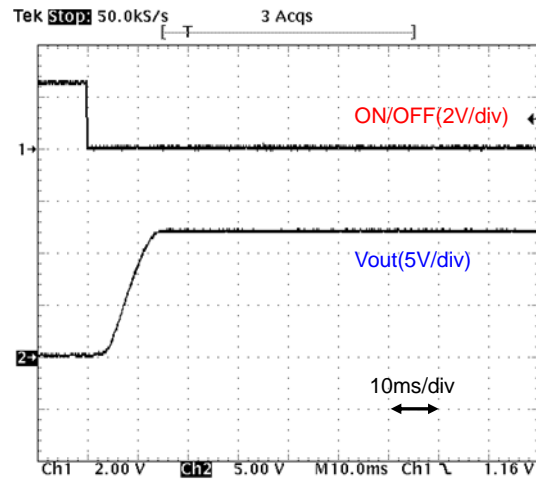
Fig.12-2-34. Start-up Waveform (Io=2A)
