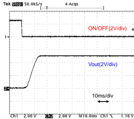
Fig.12-2-10. Start-up Waveform (Io=2A)
