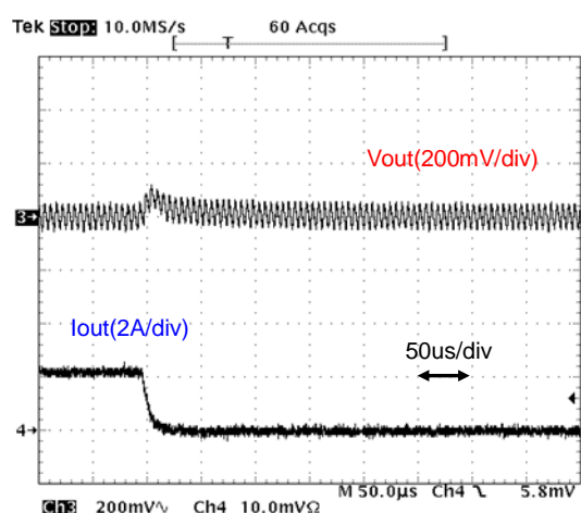
Fig.12-2-30. Load Transient Response (Io= 2A → 0)
