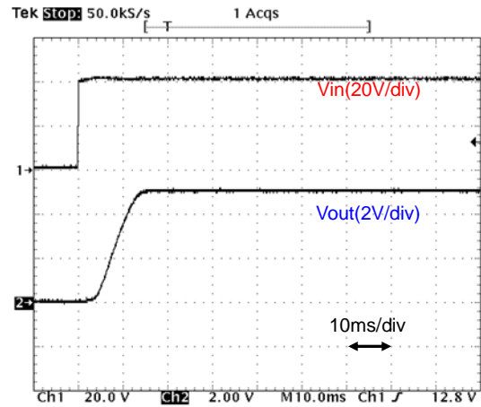
Fig.12-2-14. Start-up Waveform (Io=2A)
