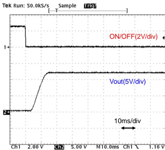
Fig.12-2-21. Start-up Waveform (Io=0A)
