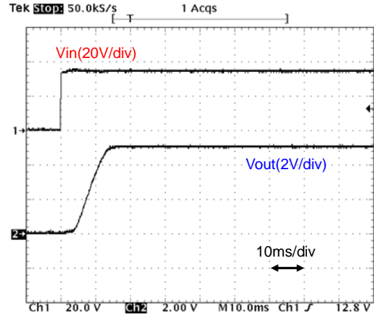
Fig.12-2-8. Start-up Waveform (Io=2A)
