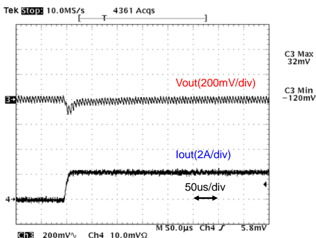
Fig.12-2-17. Load Transient Response (Io= 0 → 2A)
