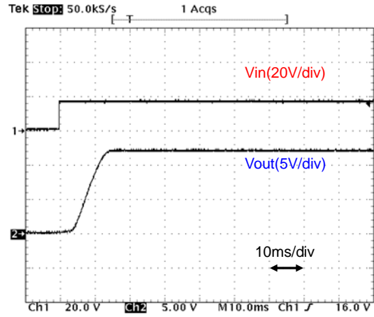
Fig.12-2-20. Start-up Waveform (Io=2A)
