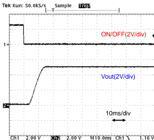
Fig.12-2-3. Start-up Waveform (Io=0A)
