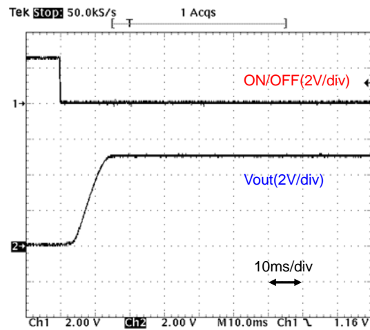
Fig.12-2-16. Start-up Waveform (Io=2A)
