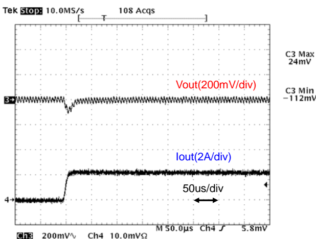
Fig.12-2-5. Load Transient Response (Io= 0 → 2A)
