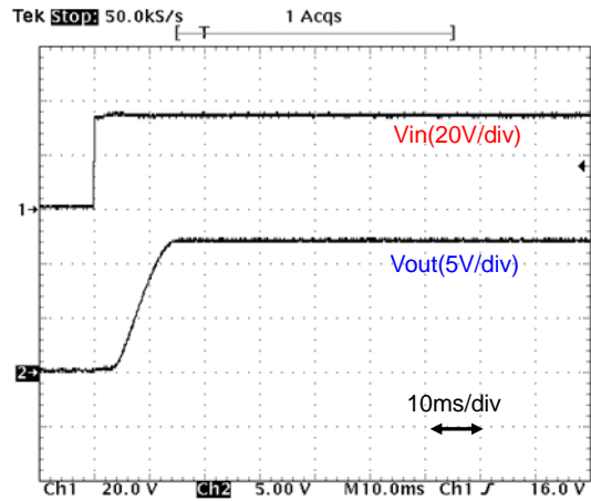
Fig.12-2-26. Start-up Waveform (Io=2A)
