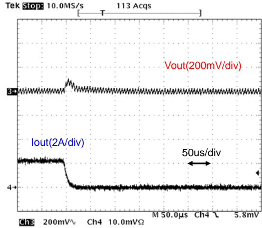
Fig.12-2-24. Load Transient Response (Io= 2A → 0)
