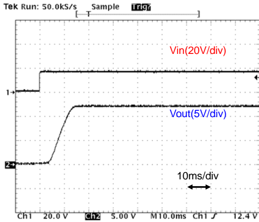
Fig.12-2-19. Start-up Waveform (Io=0A)
