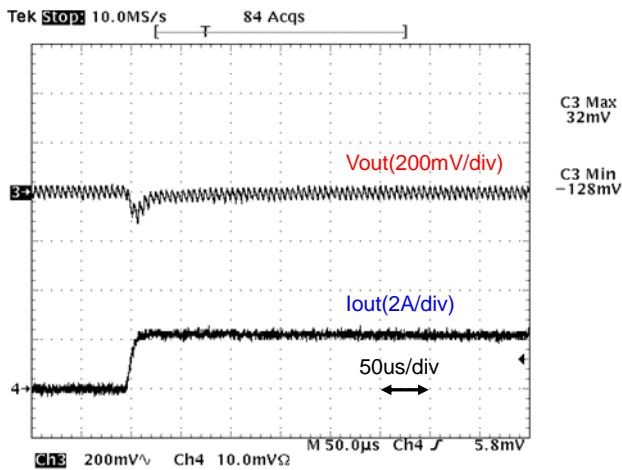
Fig.12-2-11. Load Transient Response (Io= 0 → 2A)
