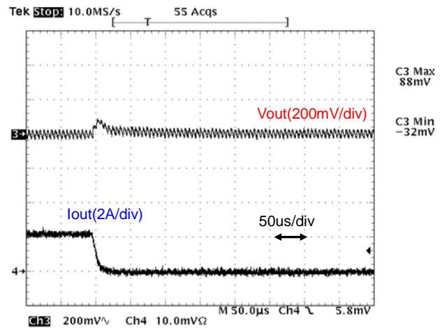
Fig.12-2-12. Load Transient Response (Io= 2A → 0)
