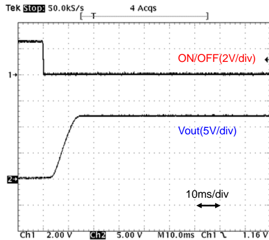
Fig.12-2-28. Start-up Waveform (Io=2A)
