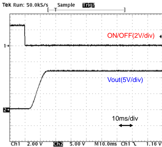
Fig.12-2-33. Start-up Waveform (Io=0A)
