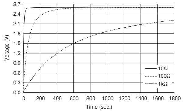
Constant Resistance Charge (@25°C)
