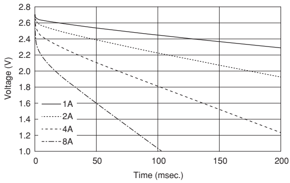
Constant Current Discharge (@25°C)
