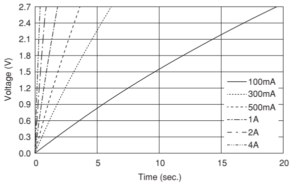
Constant Current Charge (@25°C)
