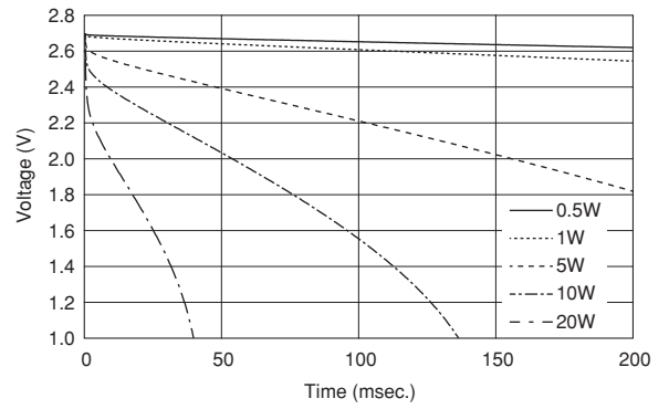
Constant Power Discharge (@25°C)
