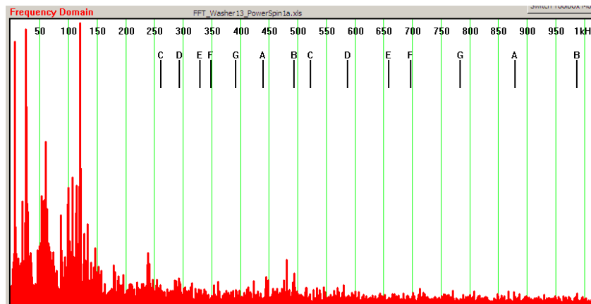
Figure 11. Washing Machine in Power Spin Mode
