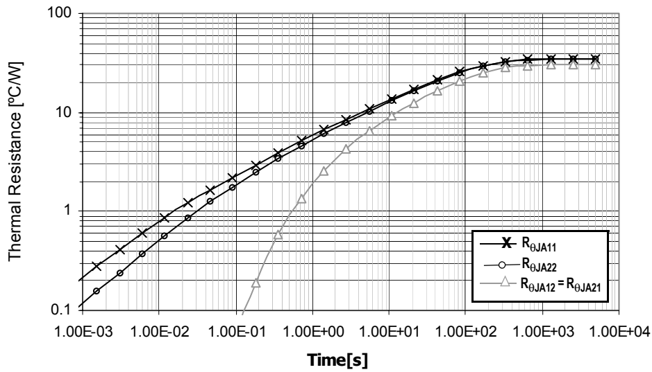
Figure 4. Transient Thermal Resistance R_{\theta JA} (1.0 W Step Response) Device on Thermal Test Board Area A = 600 (mm 2 )
