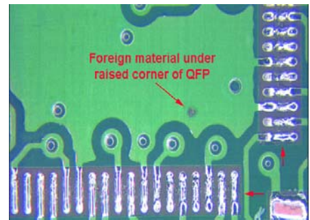
Foreign matter under QFP causing open corner leads
