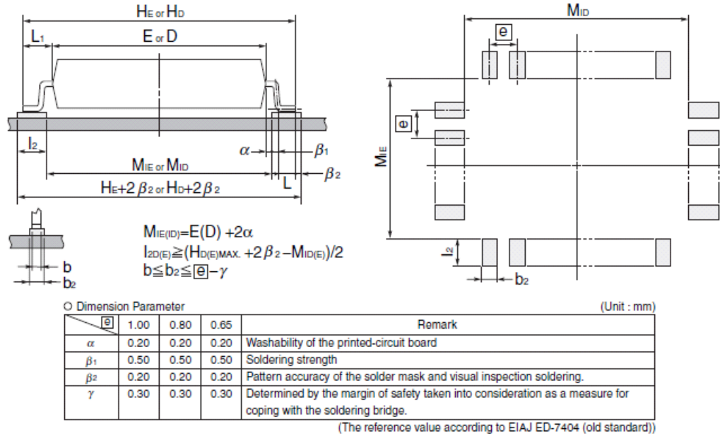
Figure 5. QFP Land Pattern Dimensions
