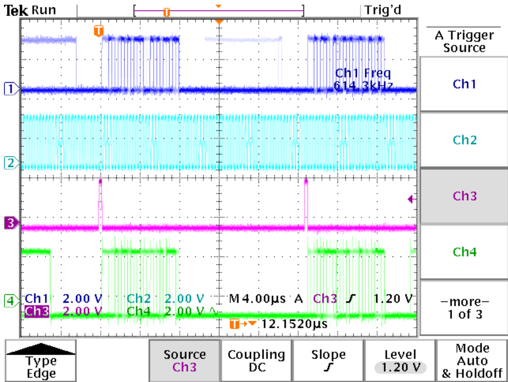
Figure 2. SGT5000 also supports 32-bit-per-channel data, using a 64-SCLK frame
