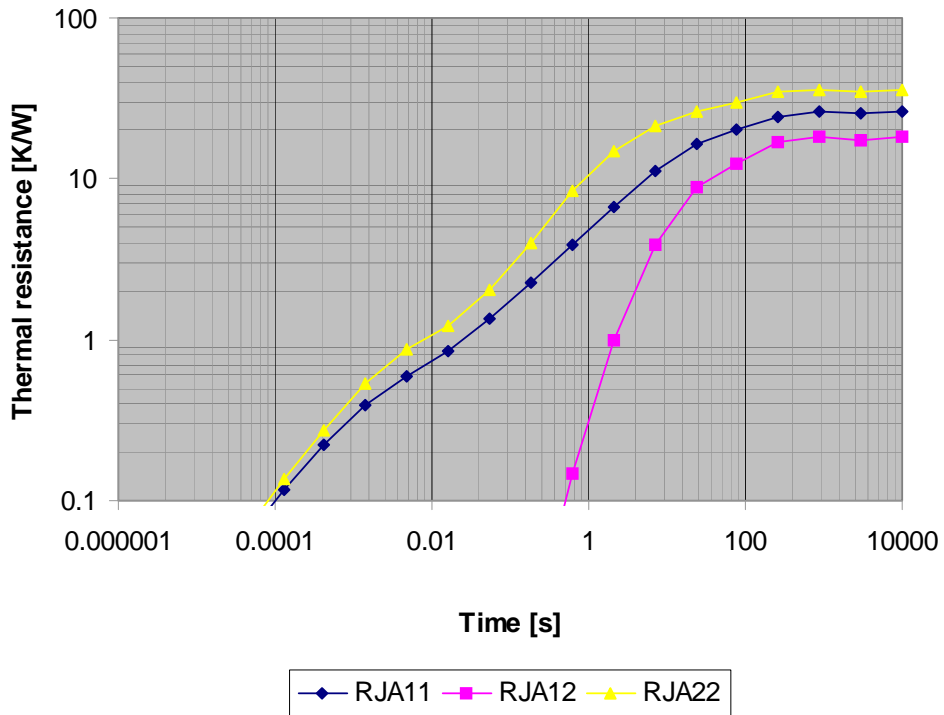
Figure 7. Transient Thermal 1W Step Response; Device on 2s2p JEDEC Standard Thermal Test Board
