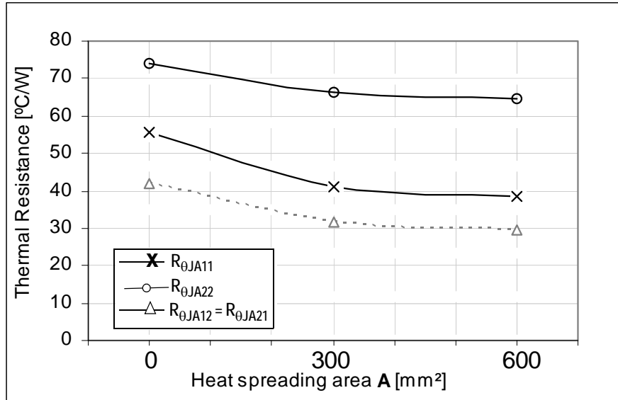
Figure 3. Device on Thermal Test Board R_{\theta JA}
