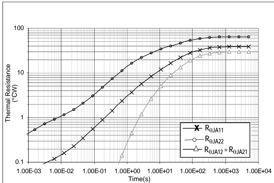
Figure 4. Transient Thermal Resistance R_{\theta JA} (1.0 W Step Response) Device on Thermal Test Board Area A = 600 (mm 2 )
